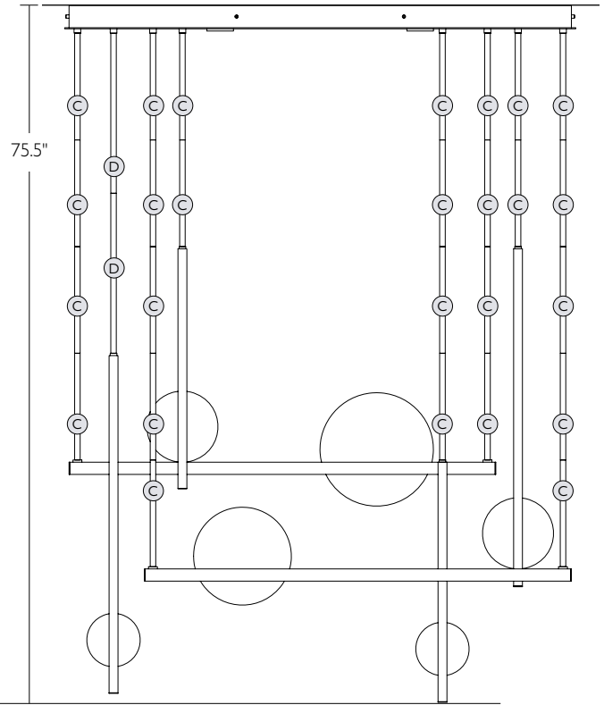
12' CEILING INSTALLATION rods used: (26) 12", (2) 18"
