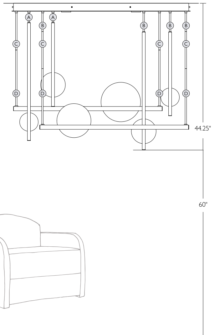
8' CEILING INSTALLATION rods used: (2) 3", (4) 6", (4) 12", (4) 18"
